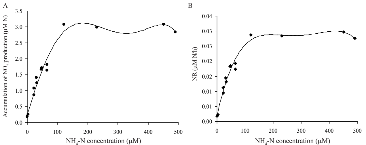
Figure 4. Accumulation of NO 2 production during 96 h incubation at various concentration of NH 4 -N (A). Nitrification rate of the Ariake seawater above mud sediment at various concentrations of NH 4 -N (B).
