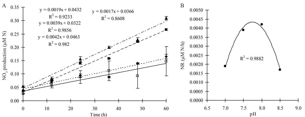
Figure 5. Nitrification rate of the Ariake seawater above mud sediment at various pHs, determined by the accumulation of NO 2 production for 60 h incubation (A). Relationship between pHs and nitrification rates of the Ariake seawater (B). ◆: 7, ■: 7.5, ▲: 8, □: 8.5, - - - - Linear (7), - - - - Linear (7.5), - - - - Linear (8), — Linear (8.5).
