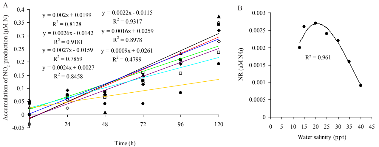
Figure 3. Nitrification rate of the Ariake seawater at various salinities, determined by the accumulation of NO 2 production for 120 h incubation (A). Relationship between water salinities and nitrification rates of the Ariake seawater (B). ◆: 13, ■: 15, ▲: 20, ○: 25, ◇: 30, □: 35, ●: 40, — Linear (13), — Linear (15), — Linear (20), — Linear (25), — Linear (30), — Linear (35), — Linear (40).
