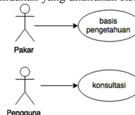
Gambar 4 Use case
