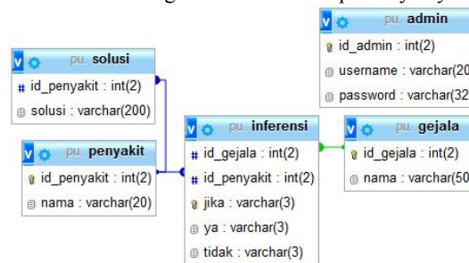
Gambar 8. Relasi basis data
