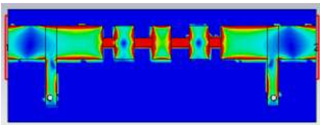
Gambar 14. Surface Current
