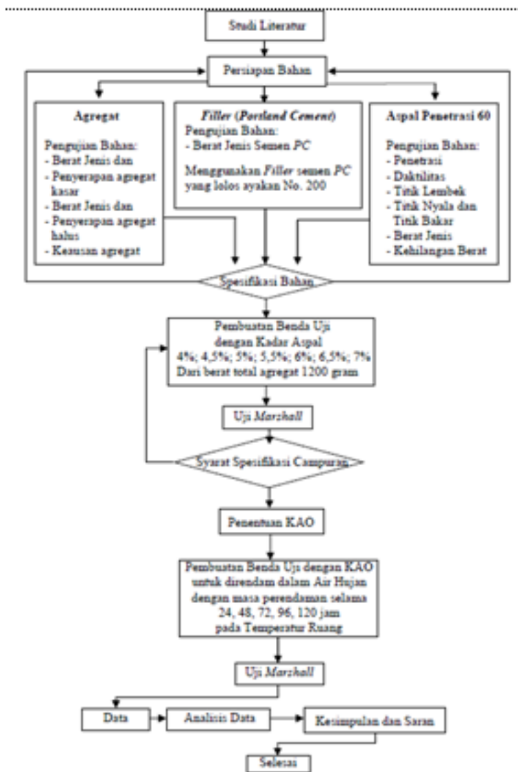
Gambar 1 Flowchart Desain
