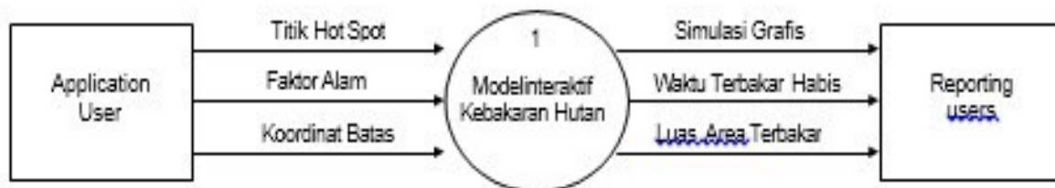
Gambar 3. DFD level 0
