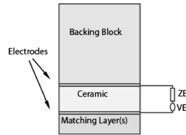
Gambar.1. Geometry transduser ultrasonik [4]
