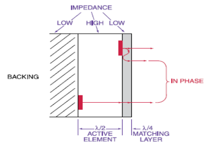
Gambar.2. Susunan matching layers [5]
