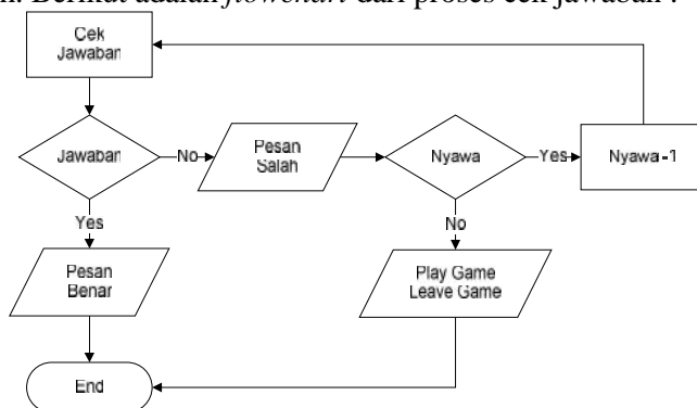
Gambar 9. Proses Cek Jawaban
