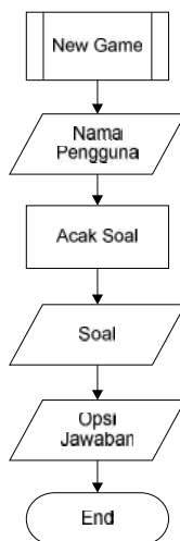
Gambar 8. Proses New Game
