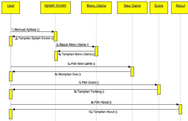
Gambar 6. Sequence Diagram Aplikasi Genius Quiz
