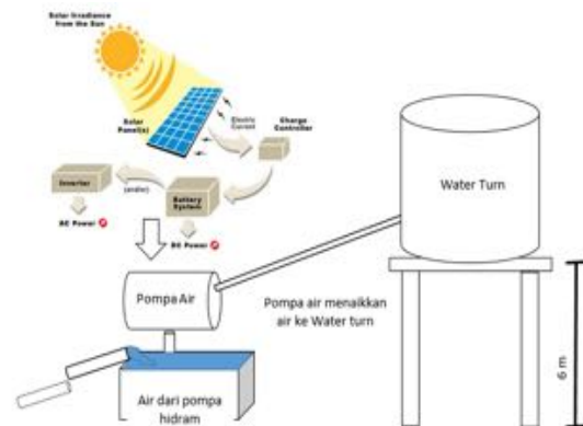
Gambar 8. Instalasi Panel Surya
