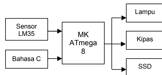
Gambar 1 – Diagram Sistem Alat
