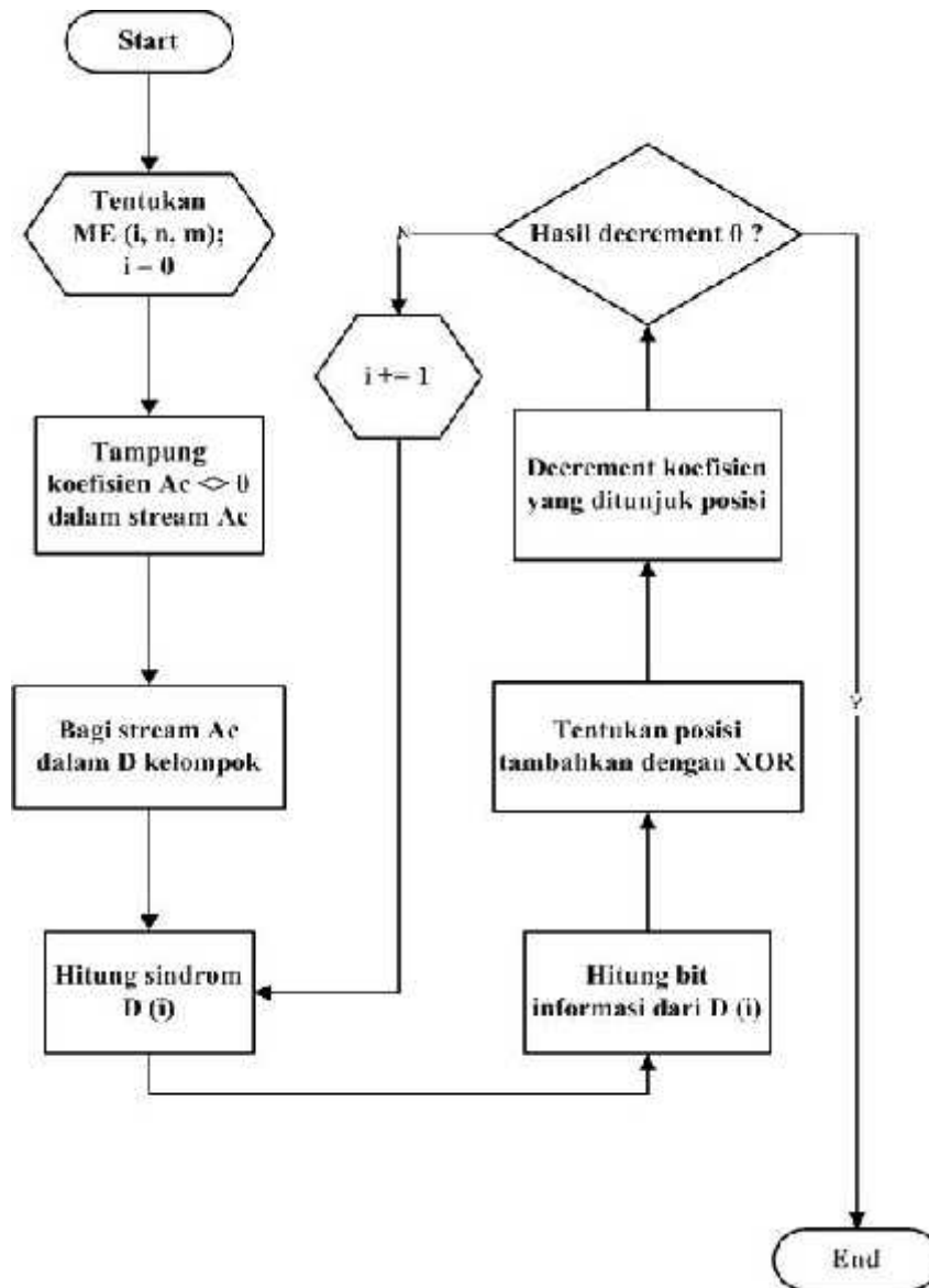
Gambar 4. Flowchart F5
