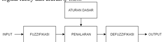
Gambar 1 Blok Diagram Logika Fuzzy (Sumber : Kurniati, Triyanto, & Rismawan, 2017)
