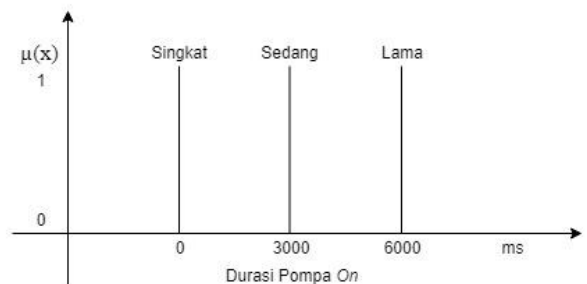
Gambar 10. Himpunan Fuzzy Durasi Pompa on Keasaman
