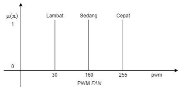
Gambar 12. Himpunan Fuzzy Nilai PWM
