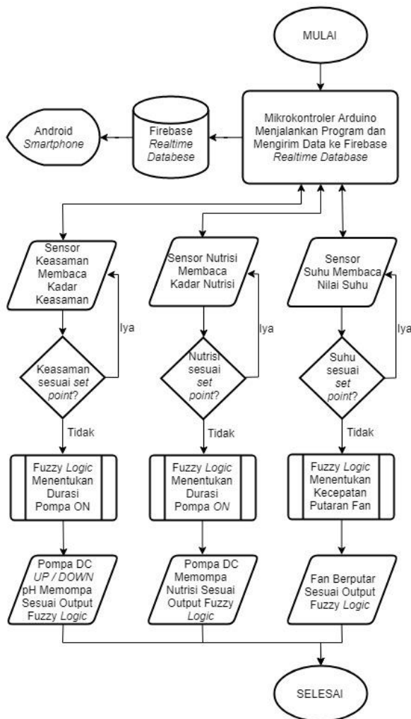
Gambar 6. Flowchat Sistem Alat
