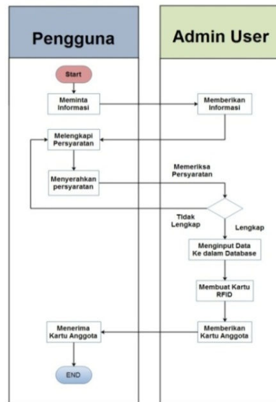
Gambar 6. Activity Diagram Proses Registrasi
