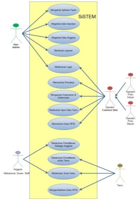
Gambar 4. Use Case Diagram Sistem Parkir
