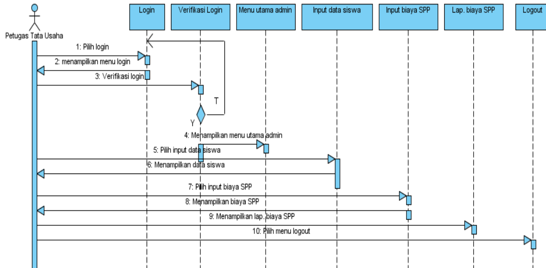
Gambar 4. Sequence Diagram
