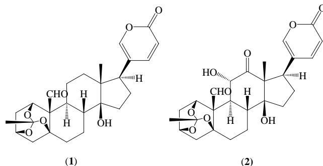
Figure 1. Structure of compounds 1 and 2.
