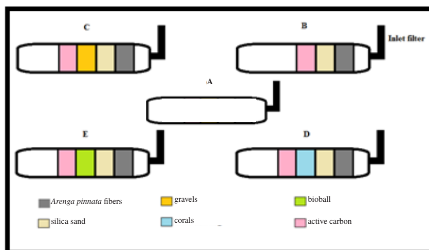
Figure 1. Filter composition layout. Treatment A uses no additional filters. Treatment B uses filters is palm fibers, silica sand, and activated carbon. Treatment C uses filters is palm fibers, silica sand, gravel, and activated carbon. Treatment D uses filters is palm fibers, silica sand, rocks, and activated carbon. Treatment E uses filters is palm fibers, silica sand, bioball, and activated carbon.
