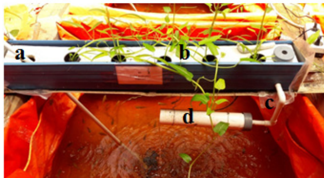
Figure 2. Aquaponics system design. (a) inlet channel, (b) Chinese spinach, (c) outlet channel, (d) filter.
