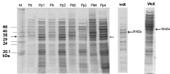
Gambar 2. Hasil SDS-PAGE ekspresi pita protein AdhF36 Salmonella typhi pada perlakuan osmolaritas (M = marker, Plt.1 = protein pelet perlakuan osmolaritas 50 mM, Pp.1 = protein pili perlakuan osmolaritas 50mM, Plt.2 = protein pelet perlakuan osmolaritas 150 mM, Pp.2 = protein pili perlakuan osmolaritas 150 mM, Plt.3 = protein pelet perlakuan osmolaritas 250 mM, Pp.3 = protein pili perlakuan osmolaritas 250 mM, Plt.4= protein pelet perlakuan osmolaritas 350 mM dan Pp .4 = protein pili perlakuan osmolaritas 350 mM)
