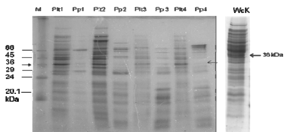
Gambar 3. Hasil SDS-PAGE protein AdhF36 Salmonella typhi pada perlakuan pH (M = protein marker, Plt1 = protein pelet perlakuan pH 4,5; Pp1 = protein pili perlakuan pH 4,5; Plt2= protein pelet perlakuan pH5,0; Pp2 = protein pili perlakuan pH5,0; Plt3 = protein pelet perlakuan pH5,5; Pp4 = protein pili perlakuan pH 5,5; Plt4 = protein pelet perlakuan pH 6,0; dan Pp4 = protein pili perlakuan pH 6,0)
