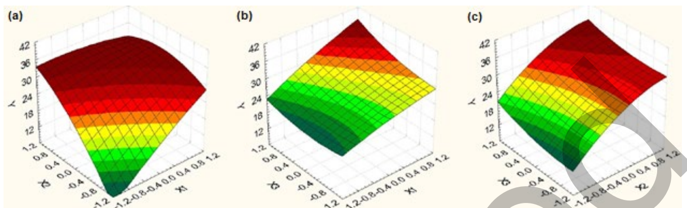
Fig 2. Response surface curve for wood vinegar yield showing the interaction between: (a) wood particle size ( X_1 ; mm) and pyrolysis temperature ( X_2 ; °C), (b) wood particle size ( X_1 ; mm) and pyrolysis time ( X_3 ; min), (c) pyrolysis temperature ( X_2 ; °C) and pyrolysis time ( X_3 ; min)
