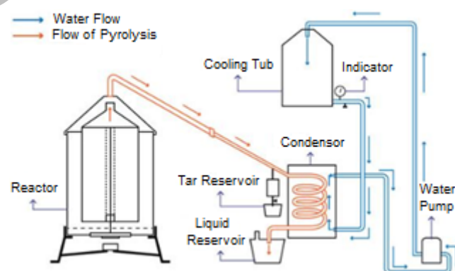
Fig 1. Pyrolysis device series scheme
